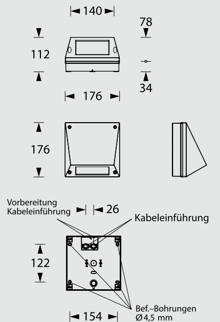
Wandmontage
