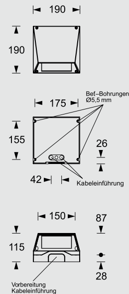
Wandmontage
